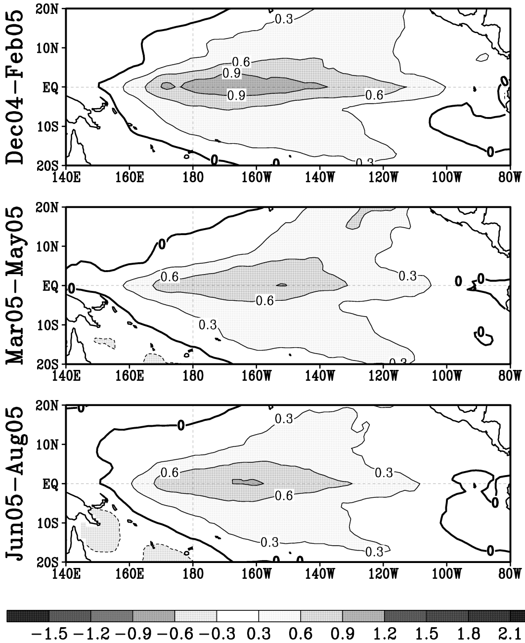
Fig. 2. Seasonal mean SST anomalies forecast by the Markov model initiated from November 2004 . The three target periods are indicated.
