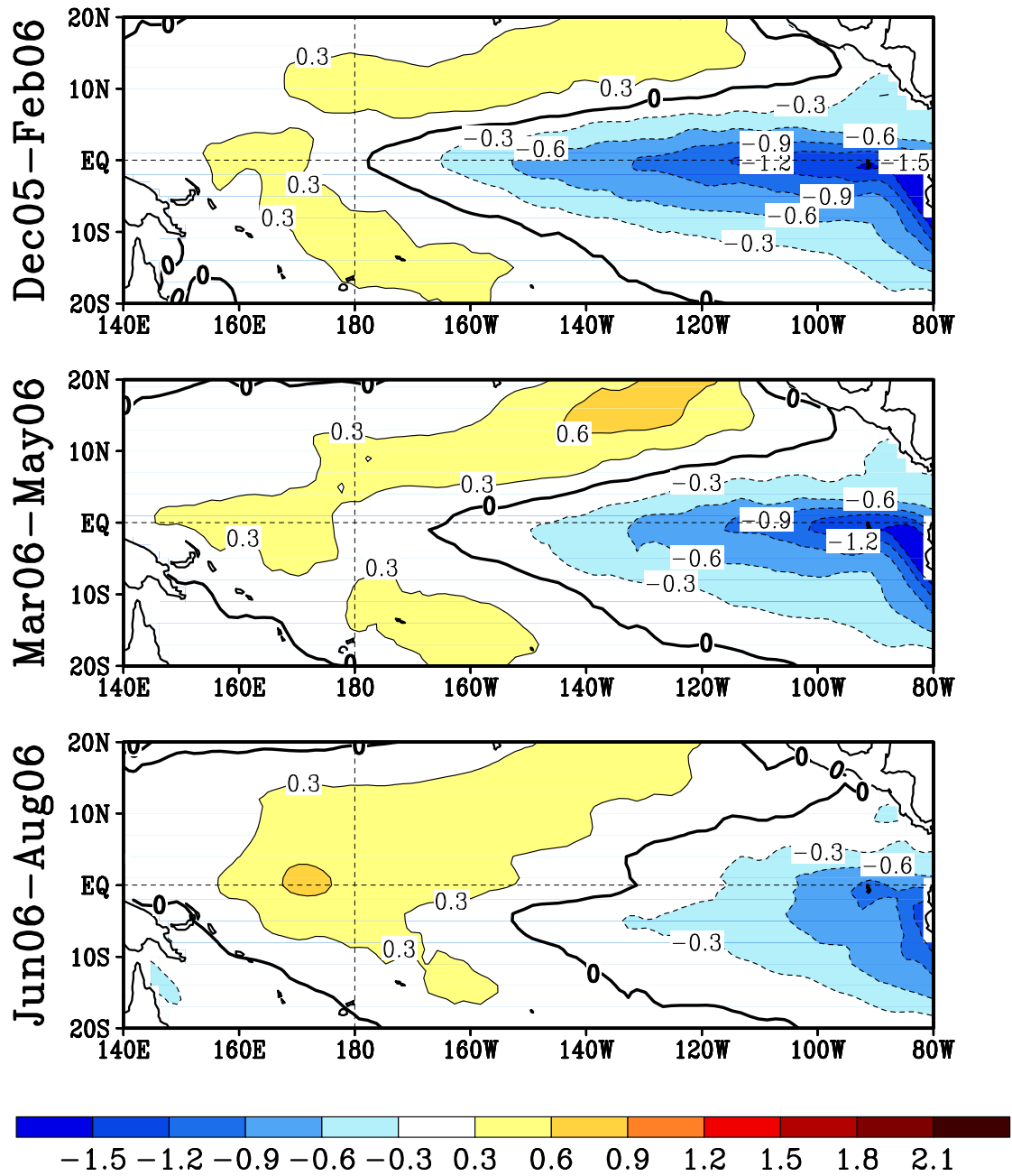
Fig. 2. Seasonal mean SST anomalies forecast by the Markov model initiated from November 2005 . The three target periods are indicated.
