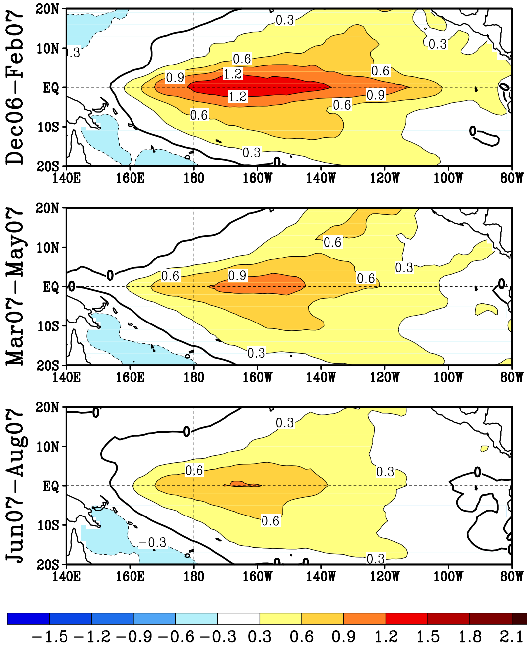
Fig. 2. Seasonal mean SST anomalies forecast by the Markov model initiated from November 2006 . The three target periods are indicated.
