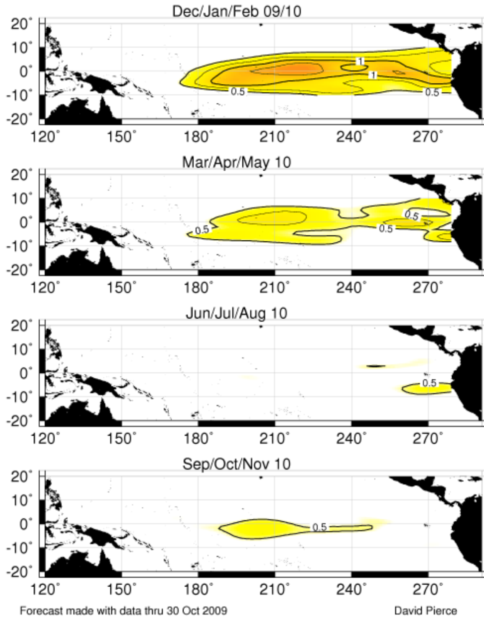
Fig. 1. Scripps/MPI hybrid coupled model (HCM-3) forecast of tropical Pacific SST anomaly (C) for DJF 2009/2010, MAM 2010, JJA 2010, and SON 2010. Observed data through 30 Oct 2009 were used to produce the forecast. Contour interval 0.25C, but contours of magnitude less than 0.5C are not shown.
