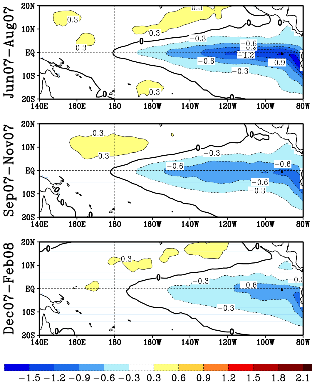
Fig. 2. Seasonal mean SST anomalies forecast by the Markov model initiated from May 2007 . The three target periods are indicated.
