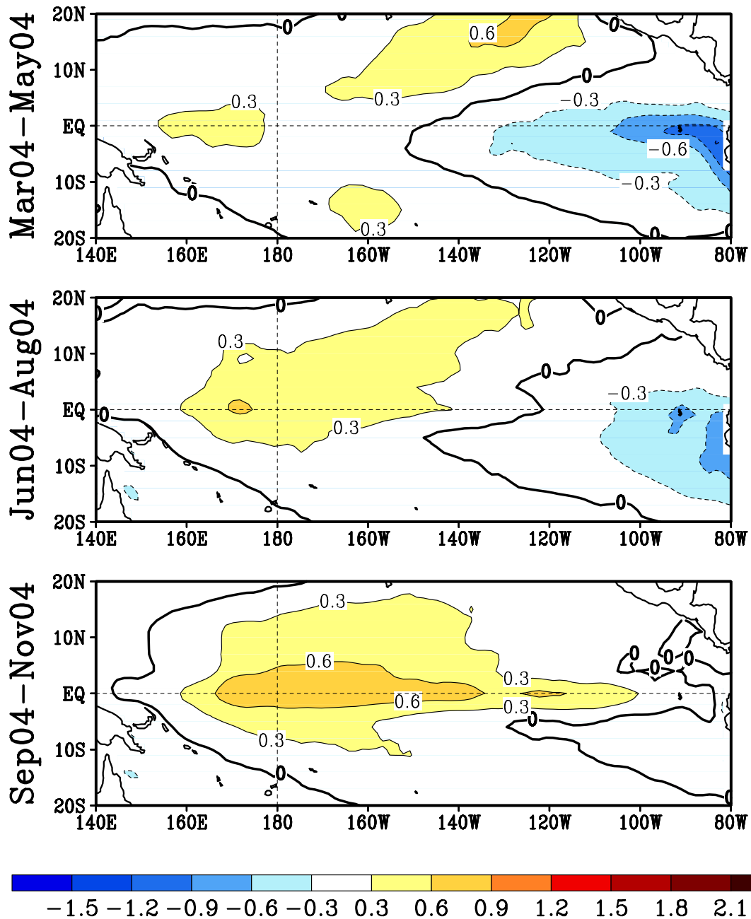
Fig. 2. Seasonal mean SST anomalies forecast by the Markov model initiated from February 2004 . The three target periods are indicated.
