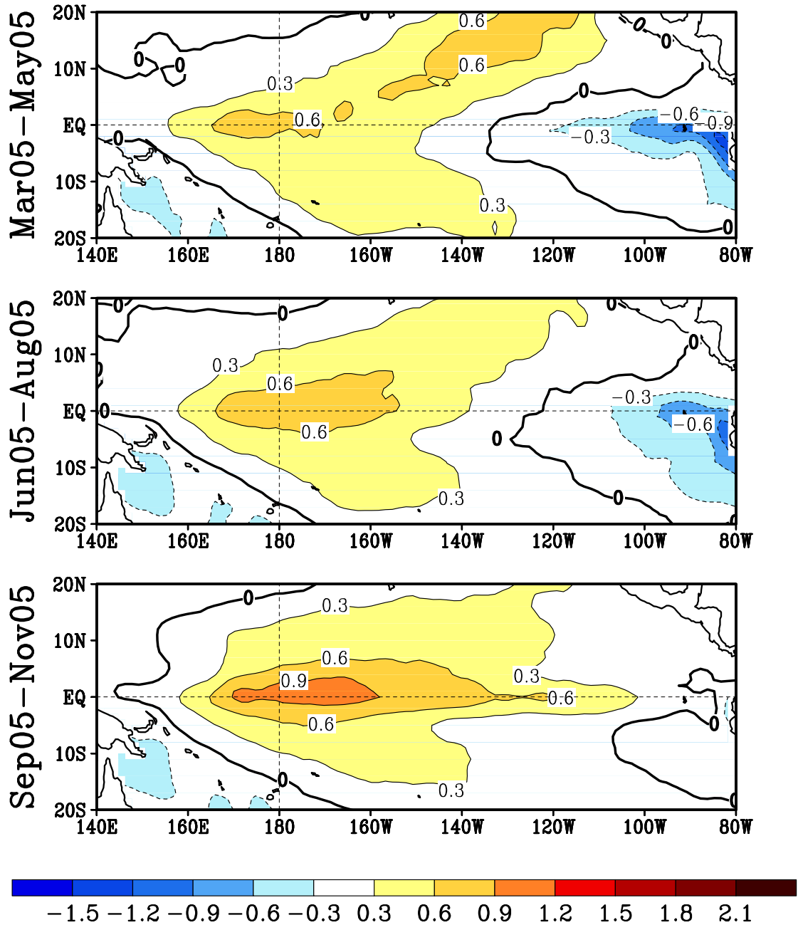
Fig. 2. Seasonal mean SST anomalies forecast by the Markov model initiated from February 2005 . The three target periods are indicated.
