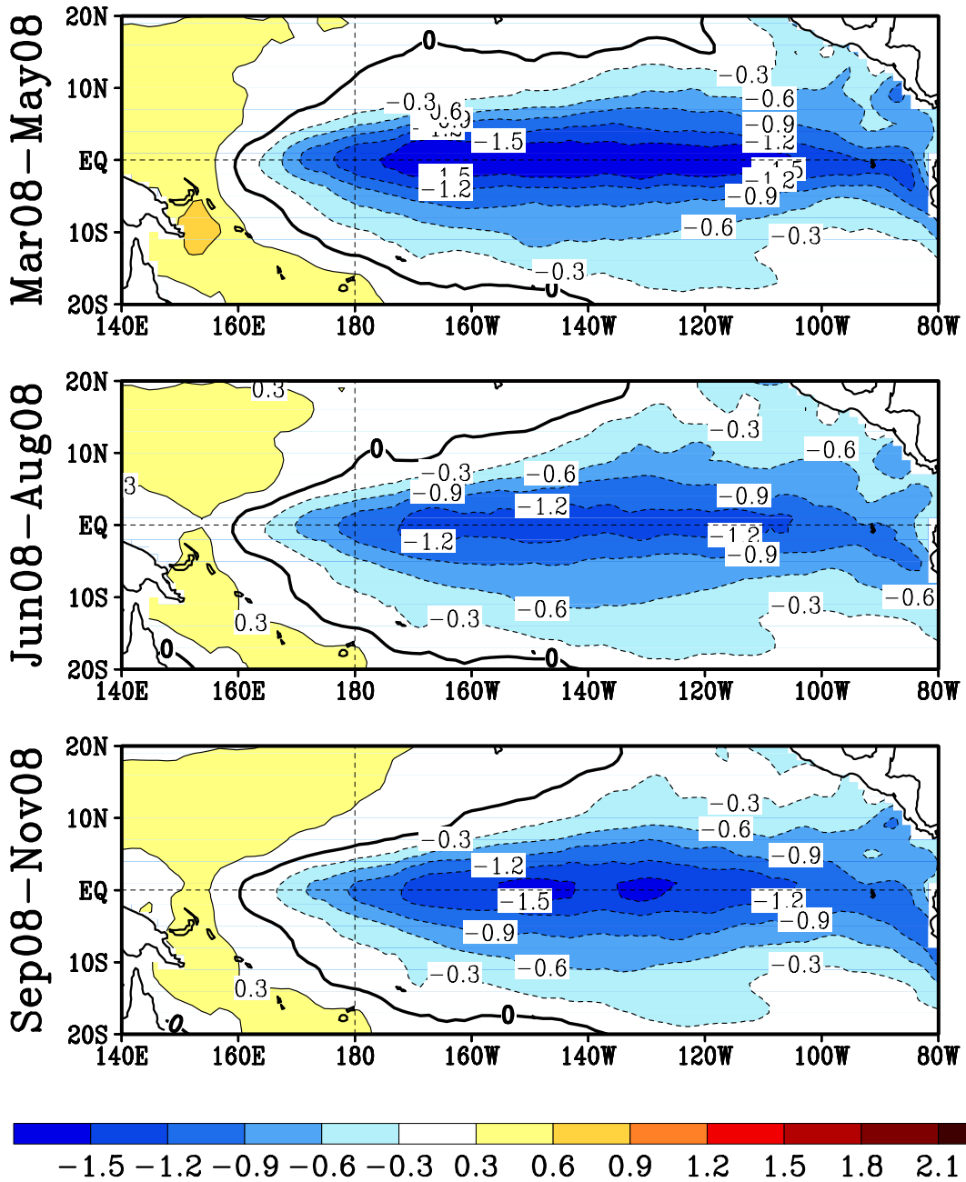
Fig. 2. Seasonal mean SST anomalies forecast by the Markov model initiated from February 2008 . The three target periods are indicated.
