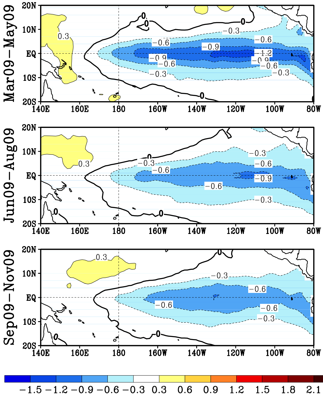
Fig. 2. Seasonal mean SST anomalies forecast by the Markov model initiated from February 2009 . The three target periods are indicated.
