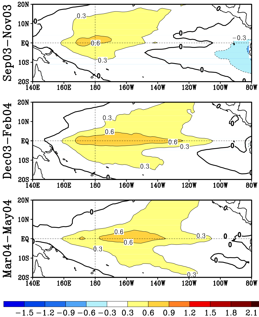
Fig. 2. Seasonal mean SST anomalies forecast by the Markov model initiated from August 2003 . The three target periods are indicated.
