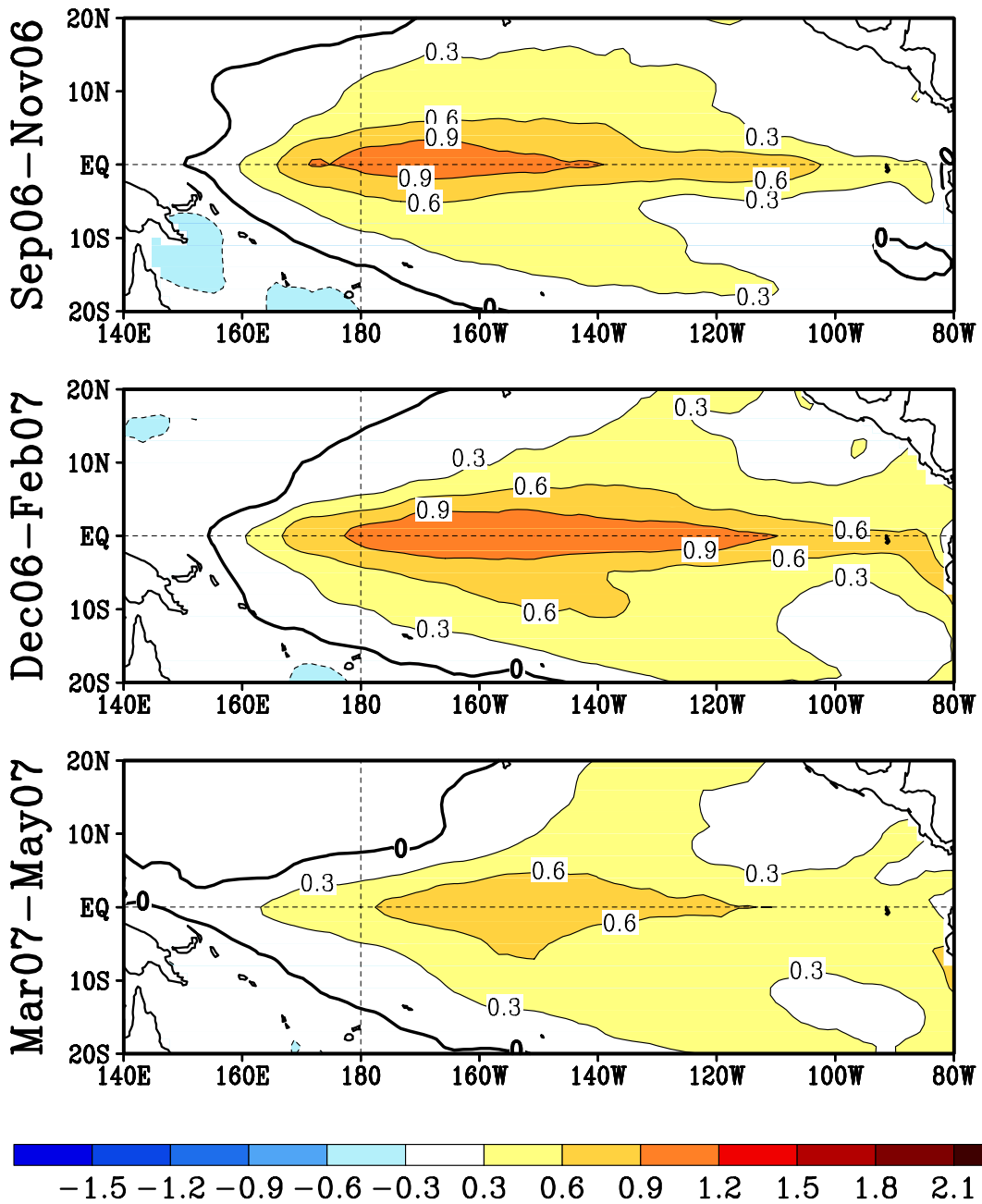
Fig. 2. Seasonal mean SST anomalies forecast by the Markov model initiated from August 2006 . The three target periods are indicated.
