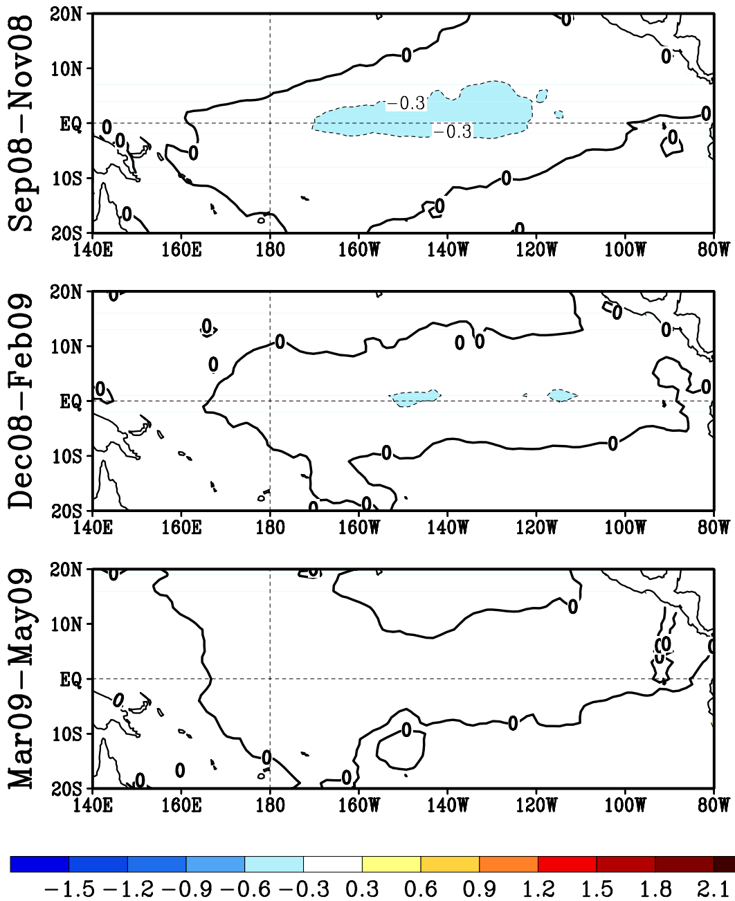
Fig. 2. Seasonal mean SST anomalies forecast by the Markov model initiated from August 2008 . The three target periods are indicated.
